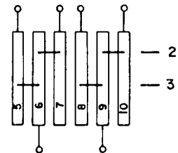
2-pole change over switch
