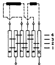
2 separate windings, one with a tap 3 or 4 switch positions
